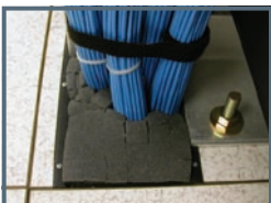
Air Dam Foam is scored into 1" sections
