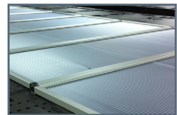
Drop-Away Panels Over Cold Aisle
